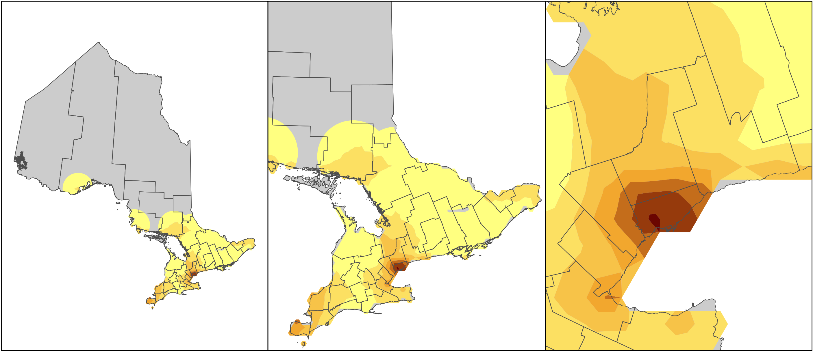
Nitrogen Dioxide (parts per billion)
