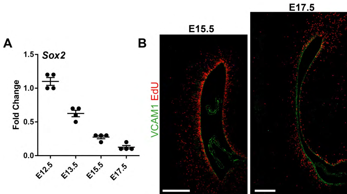
Supplemental Figure S6: Analysis of expression of Sox2 mRNA and RP proliferation in the embryonic cortex. (Related to Fig. 6). (A) qRT-PCR analysis of Sox2 mRNA in E12.5, E13.5, E15.5 and E17.5 cortices. Sox2 expression was measured relative to the reference gene Rps18 and is shown as a scatter-plot, indicating the mean \pm SEM. n = 4 independent cortical samples at each time point. (B) E15.5 or E17.5 embryos were exposed to maternally-injected EdU, and coronal cortical sections from these embryos were immunostained 6 hours later for EdU (red) and Vcam1 (green). Shown are low-magnification confocal images of the cortex (Ctx) adjacent to the lateral ventricles (LV). Scale bars = 200 \mu m.
