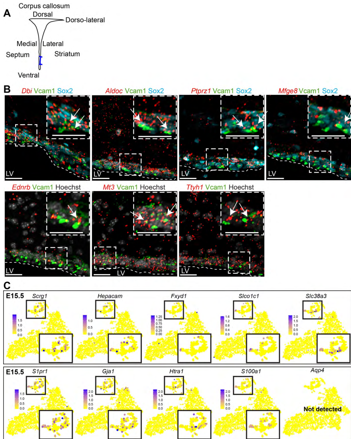
Supplemental Figure S7: Expression of genes shared between quiescent adult forebrain NSCs and embryonic RPs. (Related to Fig. 7). (A) Schematic diagram of the V-SVZ area of the adult mouse forebrain, highlighting in blue the GE-derived region that was analyzed by FISH. (B) Confocal z-stack images of coronal sections through the adult GE-derived V-SVZ analyzed by single-molecule FISH for Dbi , Aldoc , Ptprz1 , Mfge8 , Ednrb , Mt3 and Ttyh1
